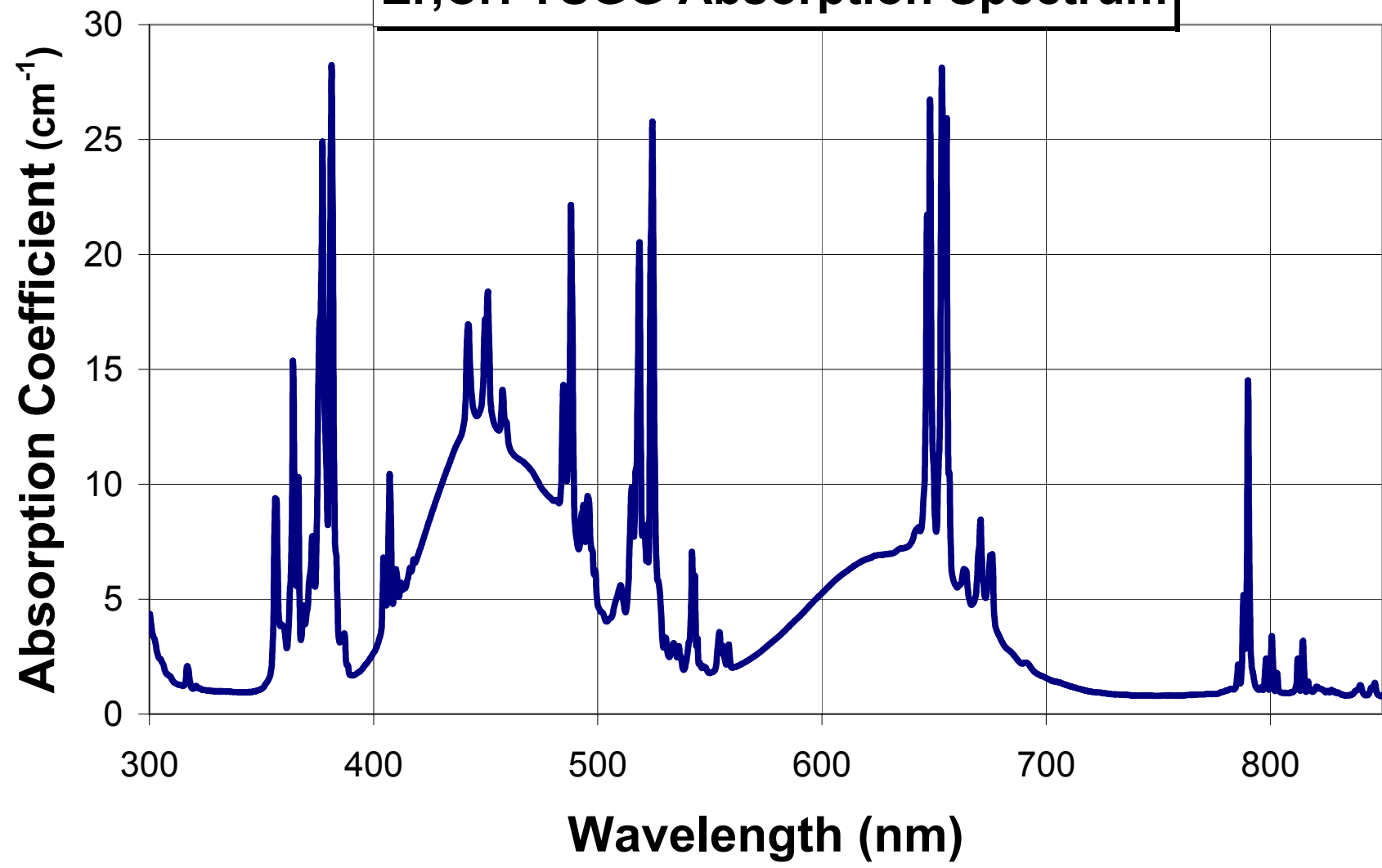
Er,Cr: YSGG Absorption Spectrum
